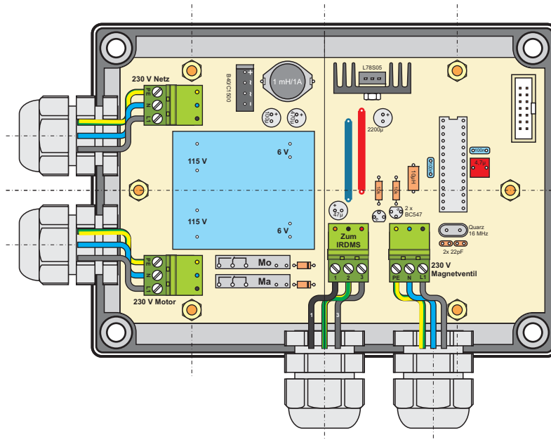
Sockel-Ebene
